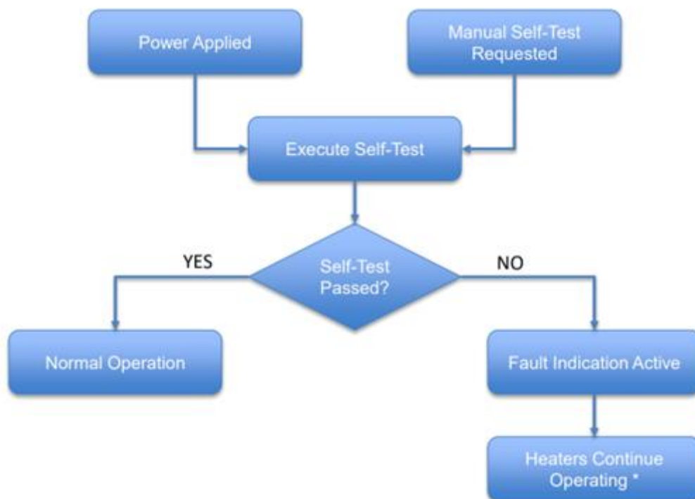
Figure 5: Self-Test Flow Chart
