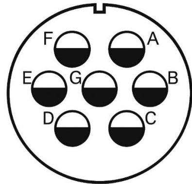
Figure 11: view – solder side
