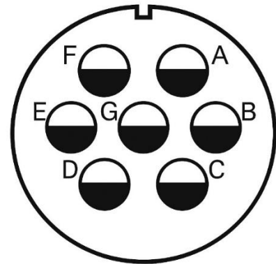
Figure 7: view – solder side
